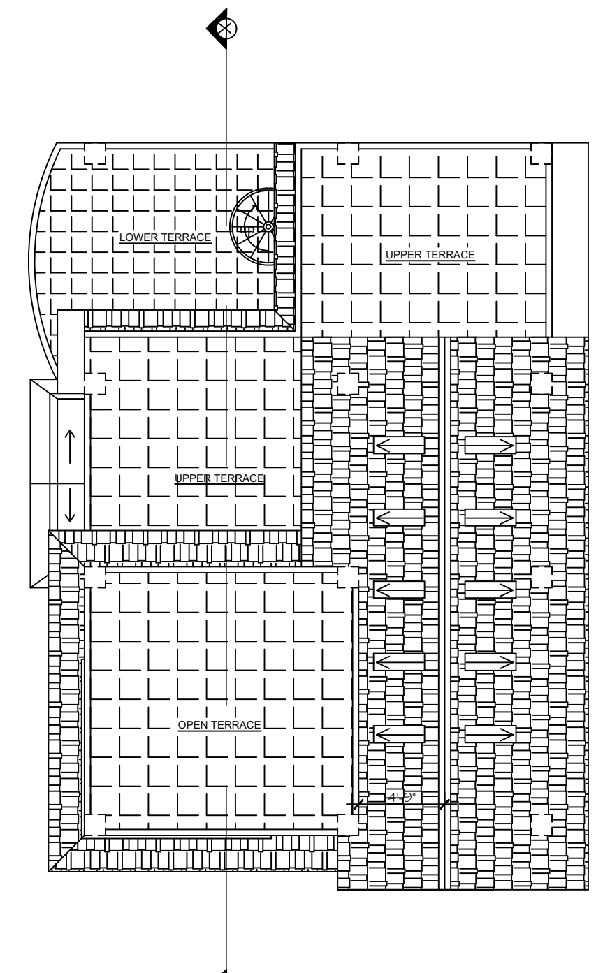
ROOF FLOOR PLAN
