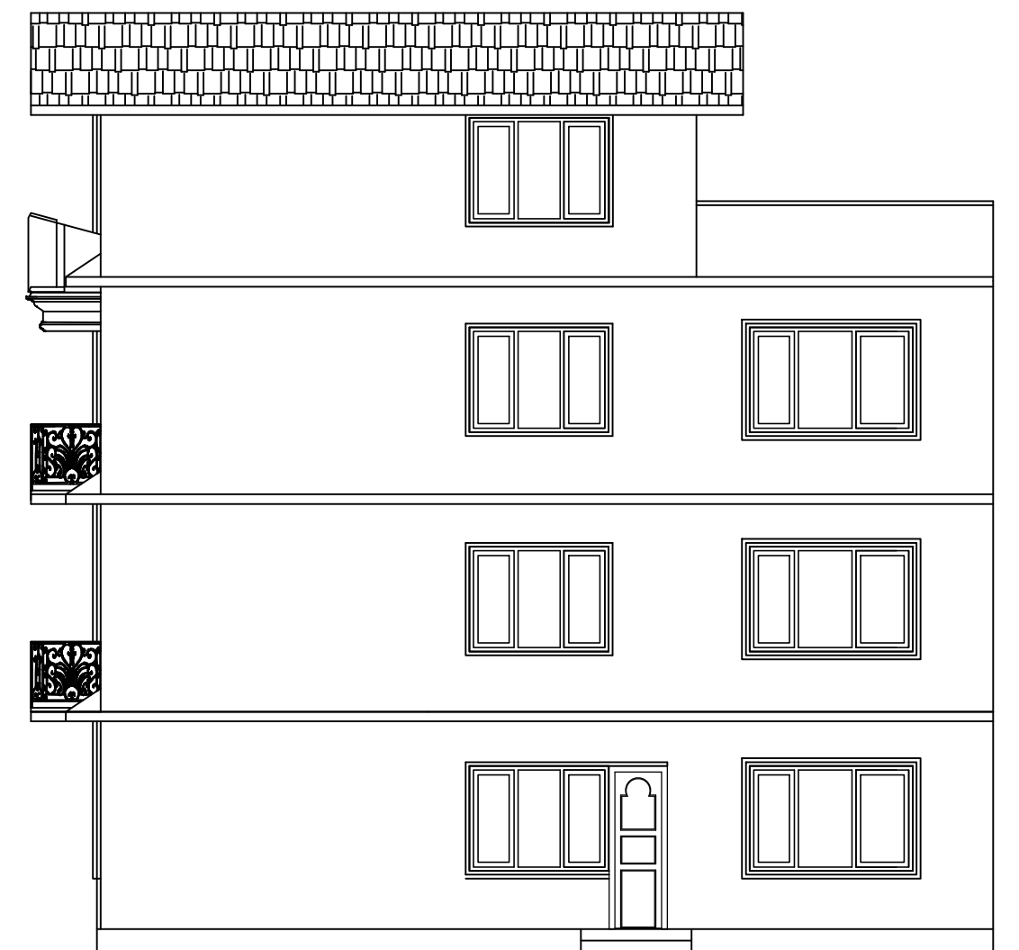
EAST ELEVATION
