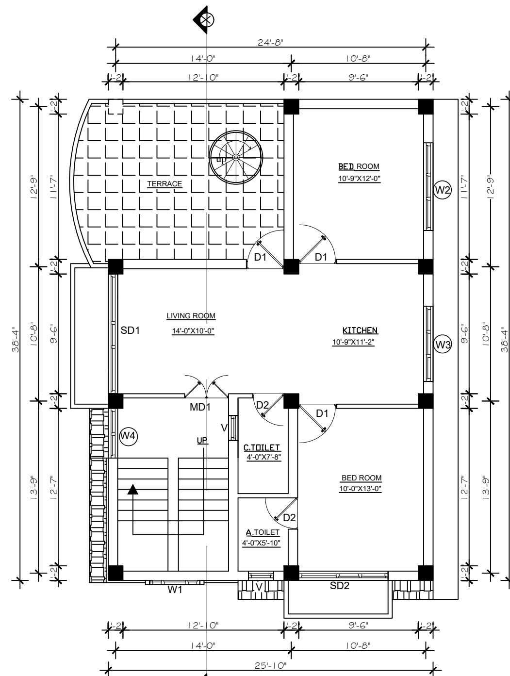
SECOND FLOOR PLAN AREA= 817.41 SQ.FT BALCONY AREA= 60.49 SQ.FT
