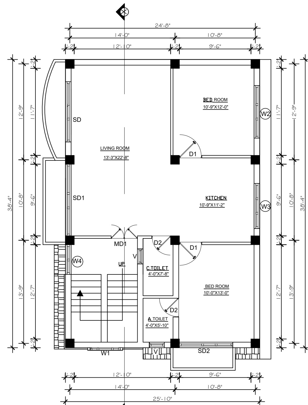
FIRST FLOOR PLAN AREA= 995.91 SQ.FT BALCONY AREA= 94.23 SQ.FT
