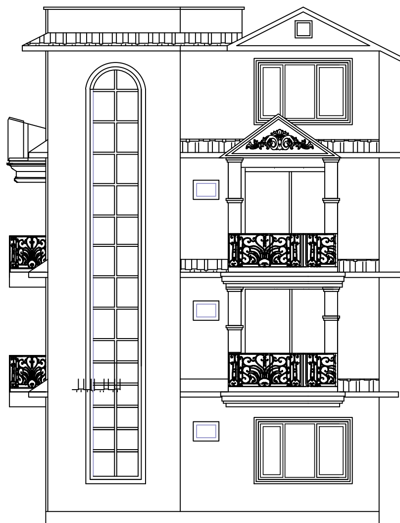
SOUTH ELEVATION
