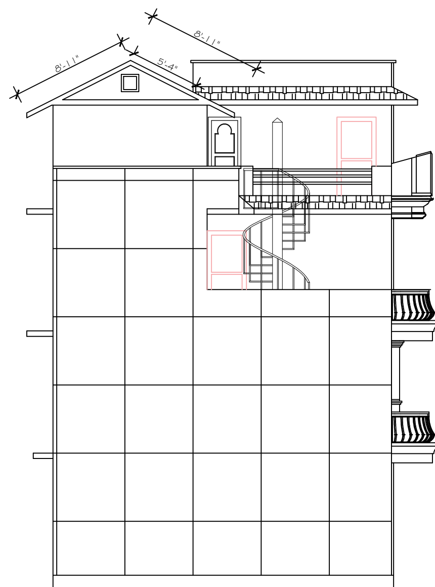
NORTH ELEVATION
