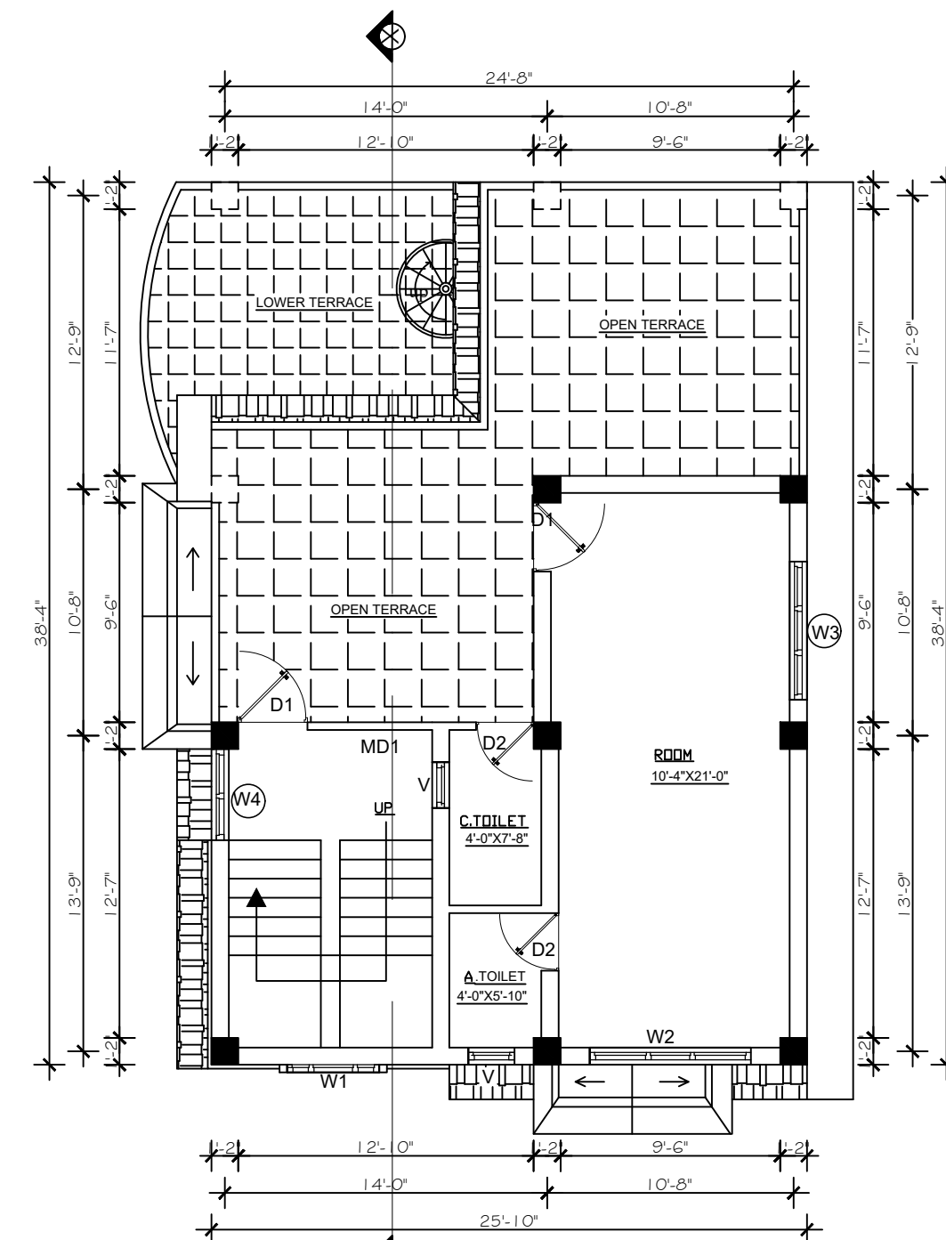
THIRD FLOOR PLAN AREA= 516.15 SQ.FT
