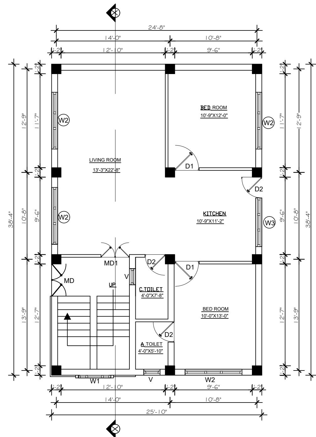
GROUND FLOOR PLAN AREA= 995.91 SQ.FT
